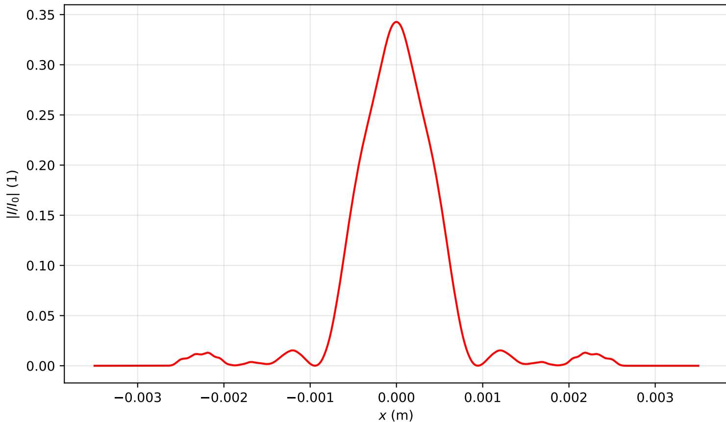
Intensity profile I(x, y = 0, z = 0.955)/I_0 , P_{in}=3.0P_{cr} , artificial time
